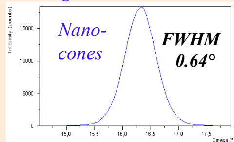
Reflectivity
