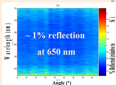
Reflectivity
